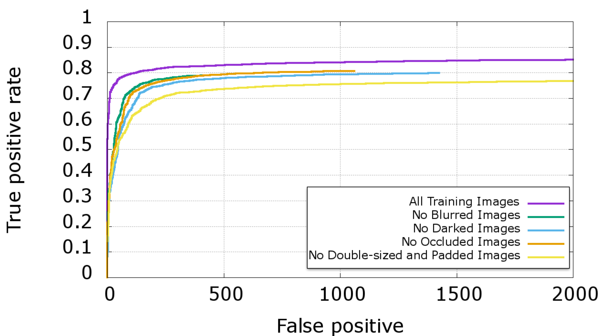
(e) Fddb Discontinuous results with different traing data
