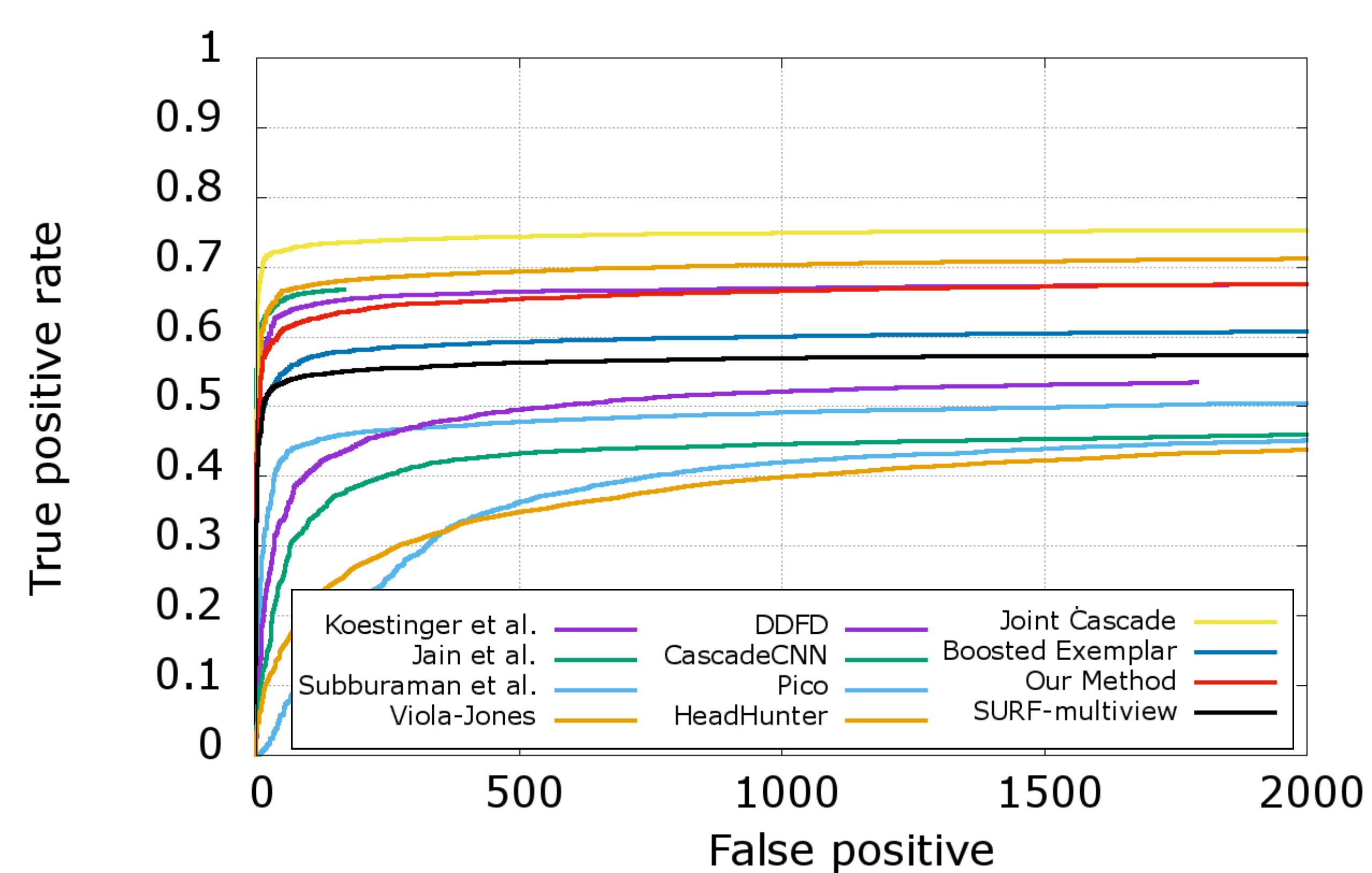
(b) Fddb Continuous results
