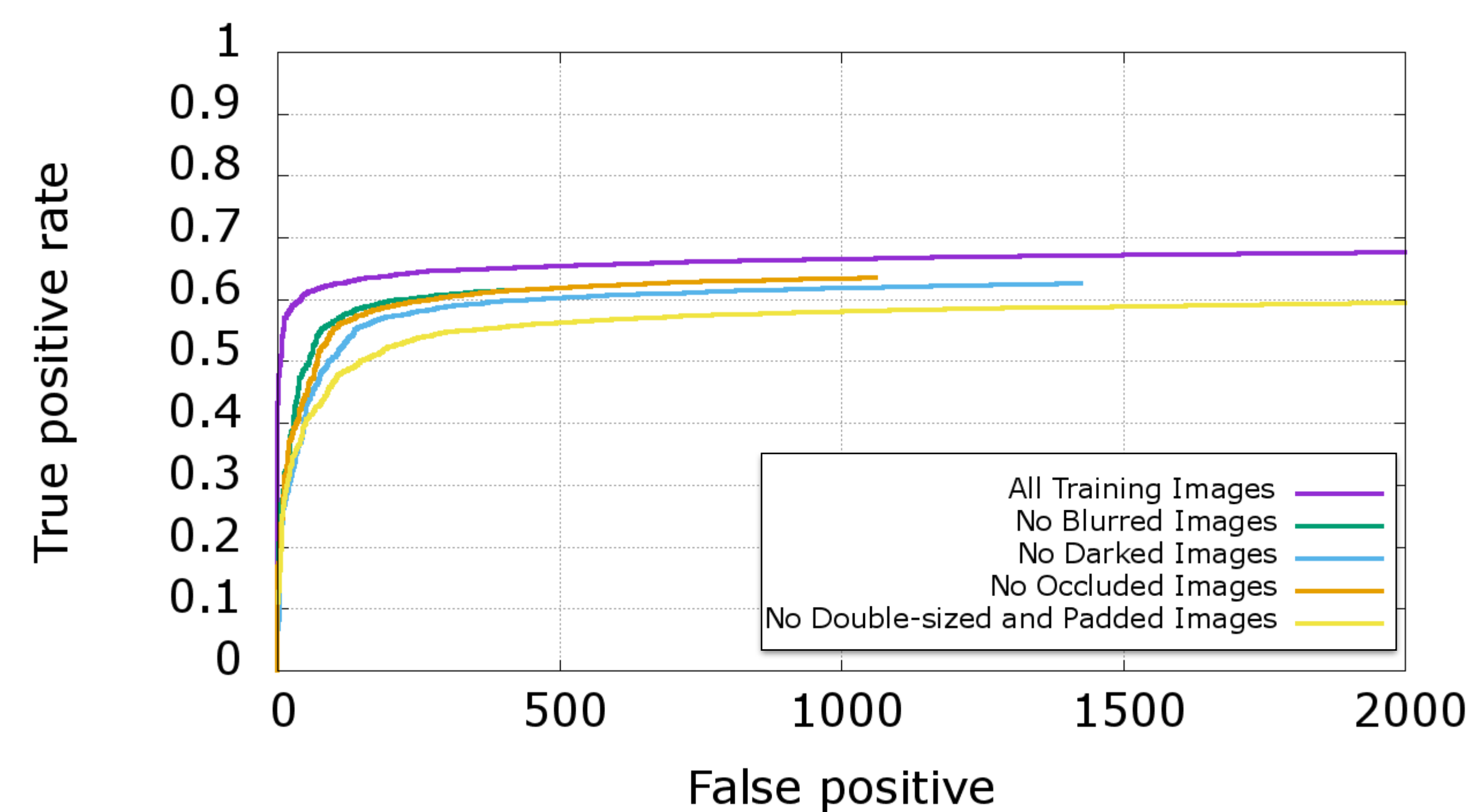
(f) Fddb Continuous results with different training data
