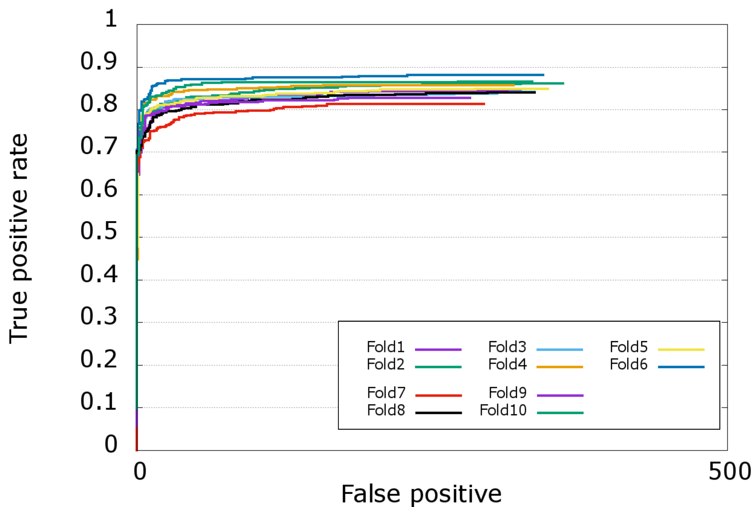
(c) Fddb Discontinuous results for each fold
