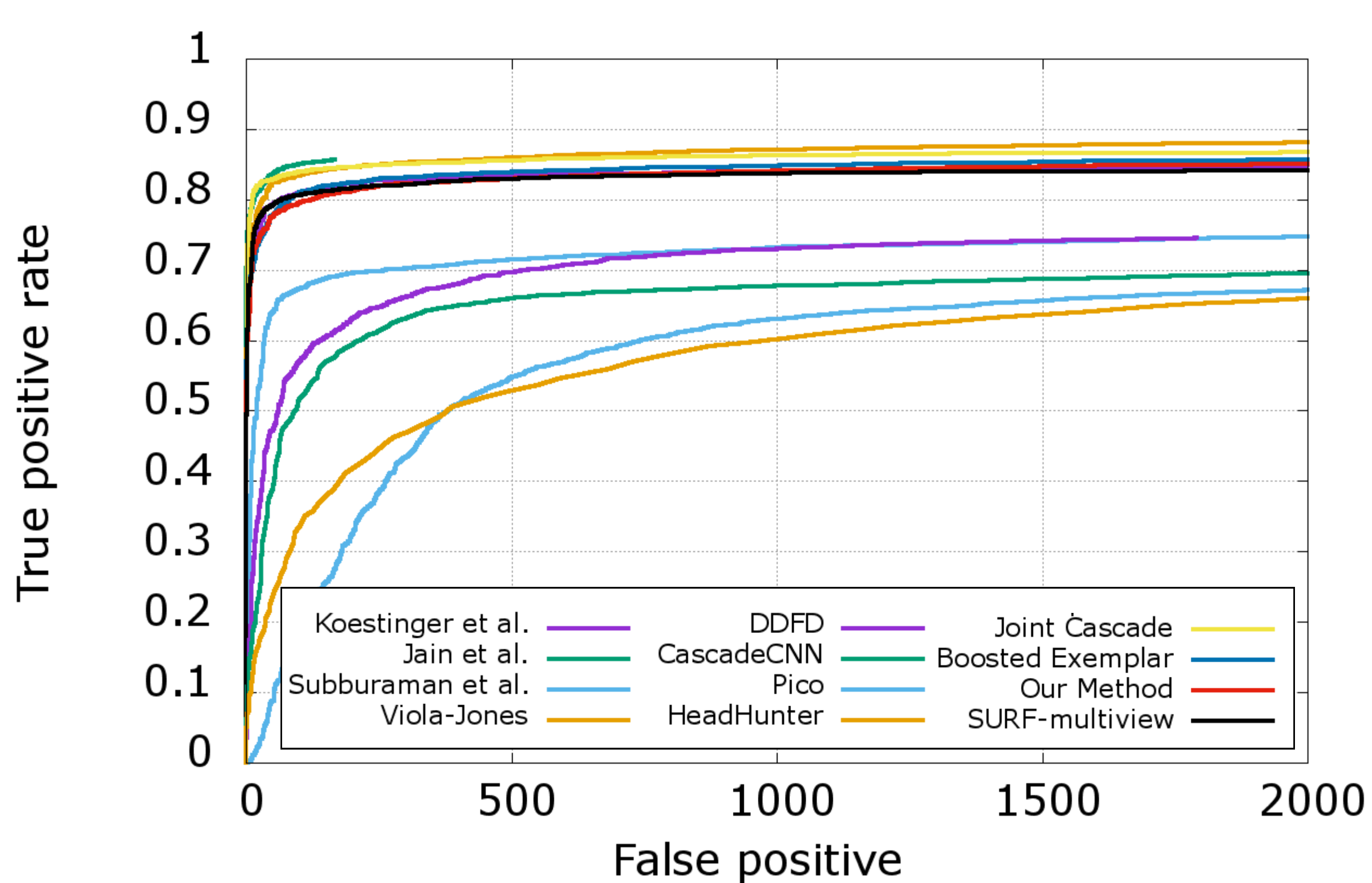
(a) Fddb Discontinuous results
