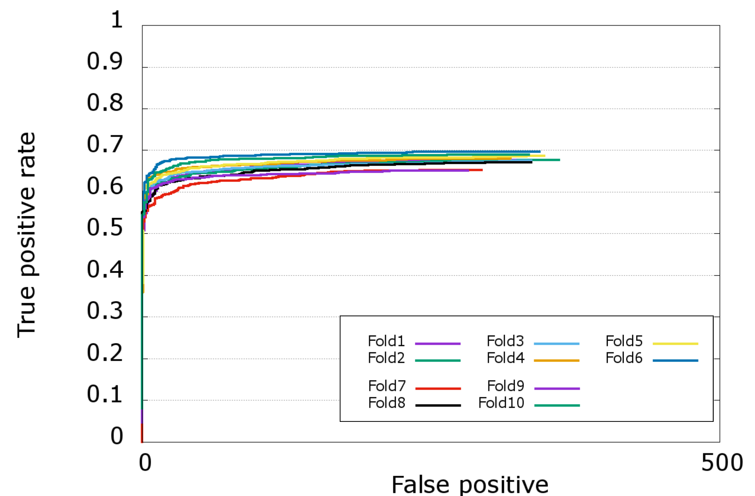
(d) Fddb Continuous results for each fold
